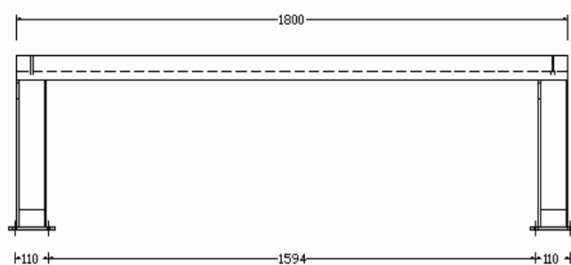
vista frontal 1/10
